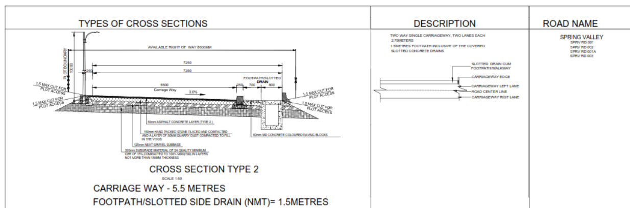
Figure 4 - Typical Road Cross Section – Spring Valley Settlement
